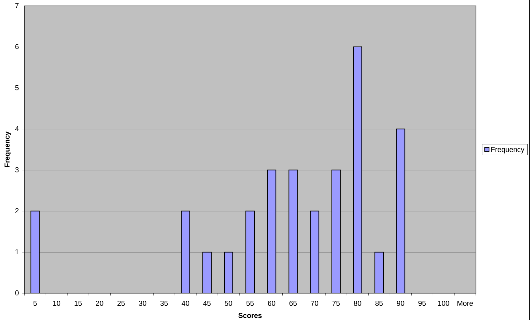
Histogram of Total Scores
